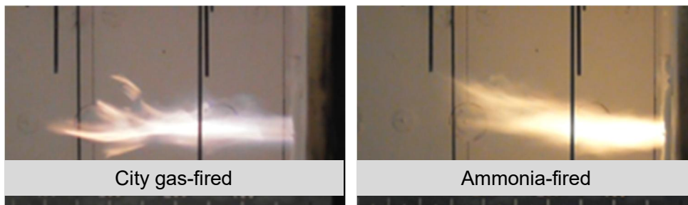
Combustion flames of the newly developed burner
